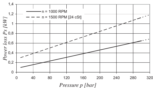
POWER LOSS HYDROMECHANICAL (TYPICAL)
