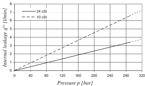
INTERNAL LEAKAGE (TYPICAL)
