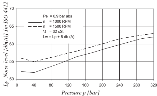
NOISE LEVEL (TYPICAL) - T7B - B10
