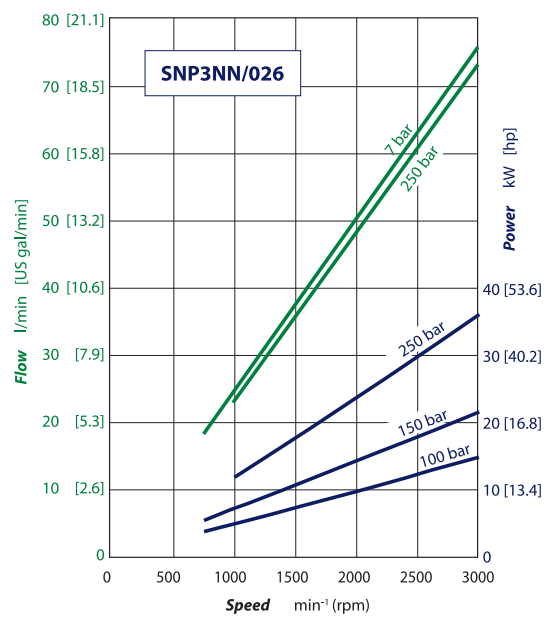
SNP3NN/026 pump performance graph
