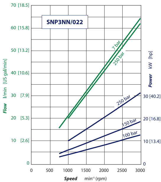
SNP3NN/022 pump performance graph
