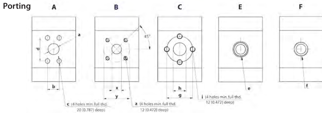
Ports dimensions
