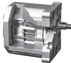
SNP3NN 01BA (cut away)
