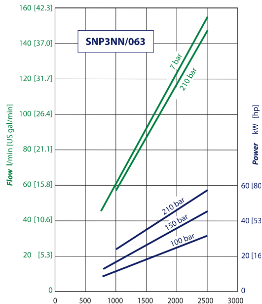
SNP3NN/063 pump performance graph
