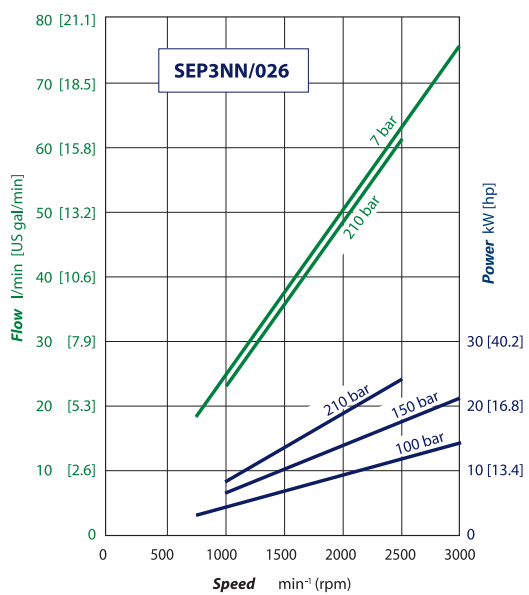
SEP3NN/026 pump performance graph
