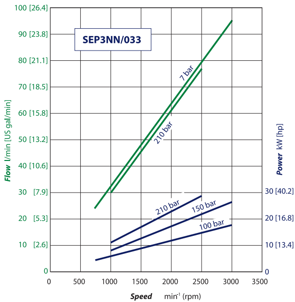
SEP3NN/033 pump performance graph
