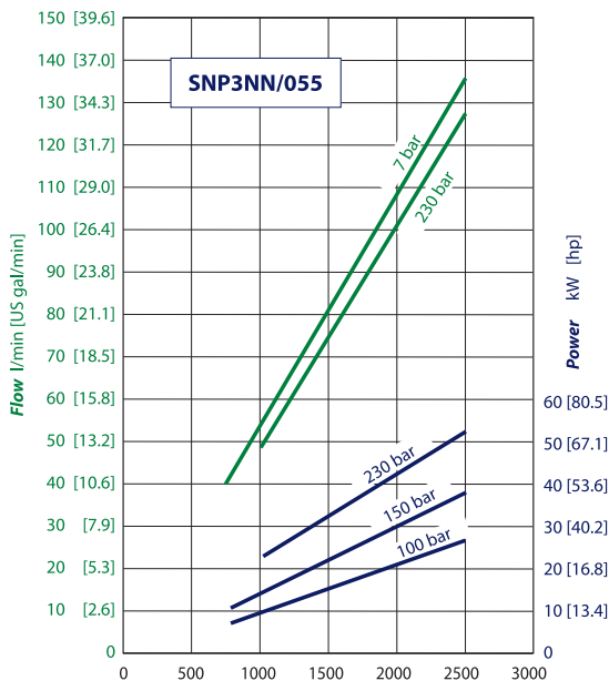
SNP3NN/055 pump performance graph
