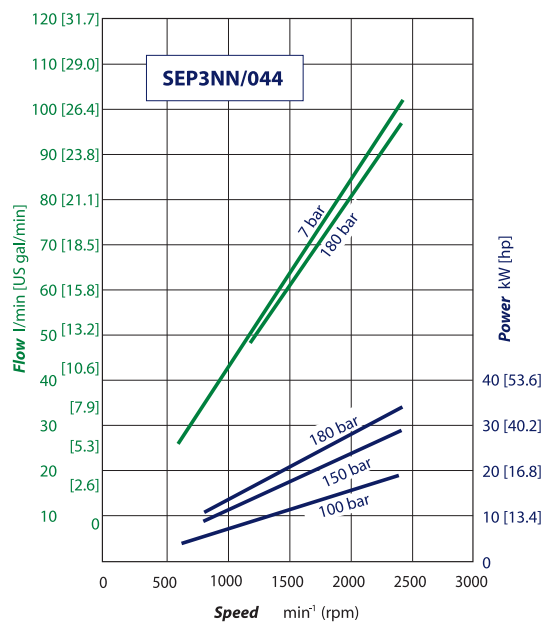
SEP3NN/044 pump performance graph
