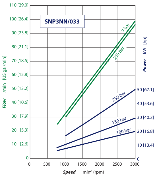
SNP3NN/033 pump performance graph
