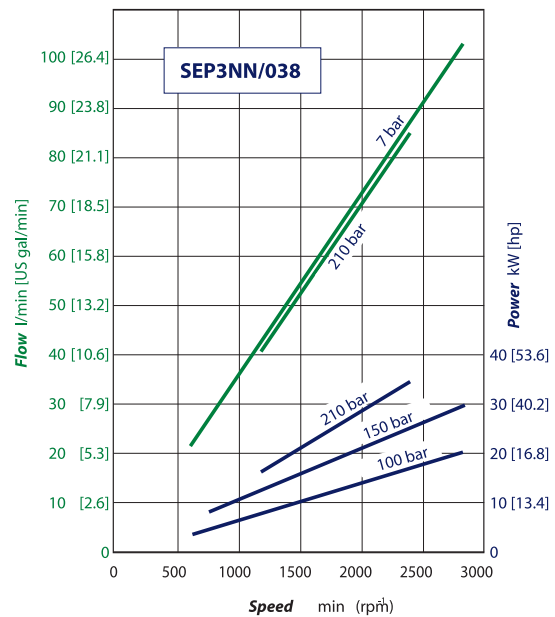
SEP3NN/038 pump performance graph
