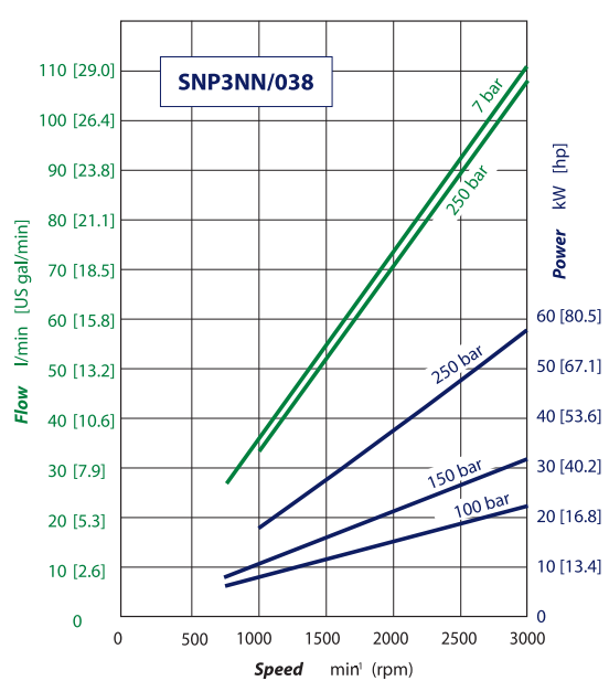
SNP3NN/038 pump performance graph
