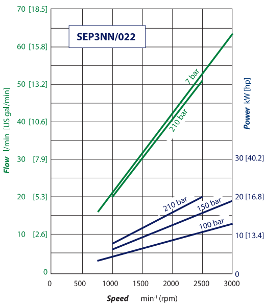
SEP3NN/022 pump performance graph
