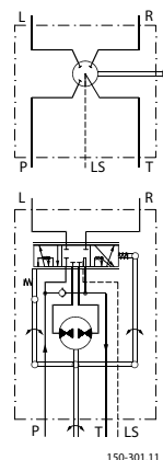
Top: Danfoss diagram; bottom: CETOP diagram
