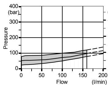
Spring nr. 2 (green band)
