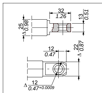
Spool dimension
