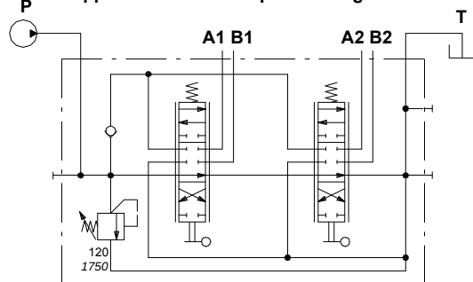
Upper inlet and outlet ports configuration
