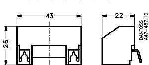
RC-Glied für Schütze CI 6, 9, 12, 15, 16, 20, 25, 30
