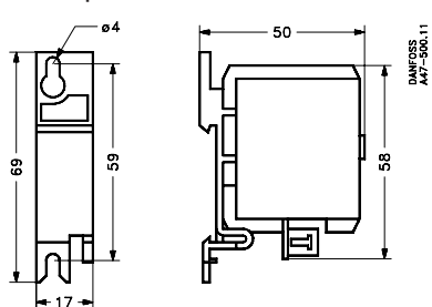
RC-Glied für Schütze CI 6, 9, 12, 15, 16, 20, 25, 30
