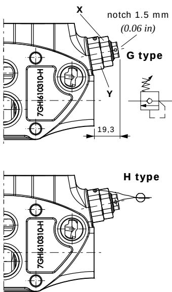
UG4 setting range From 180 to 350 bar (from 2600 to 5100 psi)
