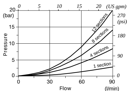
P \Rightarrow T pressure drop
