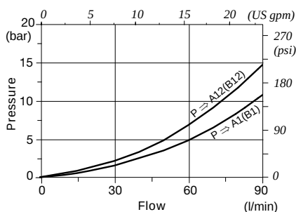
P \Rightarrow A(B) pressure drop
