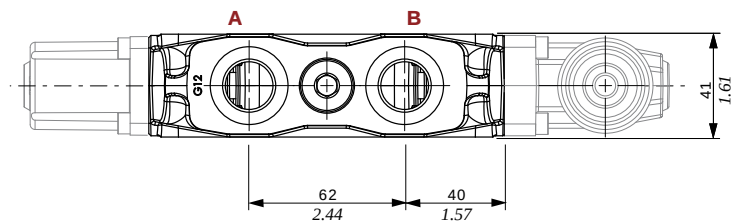
Q type Without port valve arrangement
