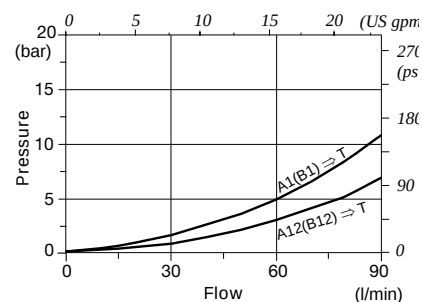
A(B) \Rightarrow T pressure drop
