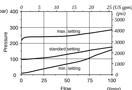
UG3 setting range From 100 to 250 bar (from 1450 to 3600 psi)
