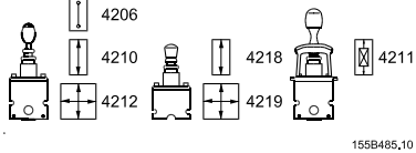
PVRES, electrical control unit, 155B...
