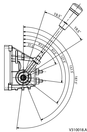
Base with an angle of 37.5°
