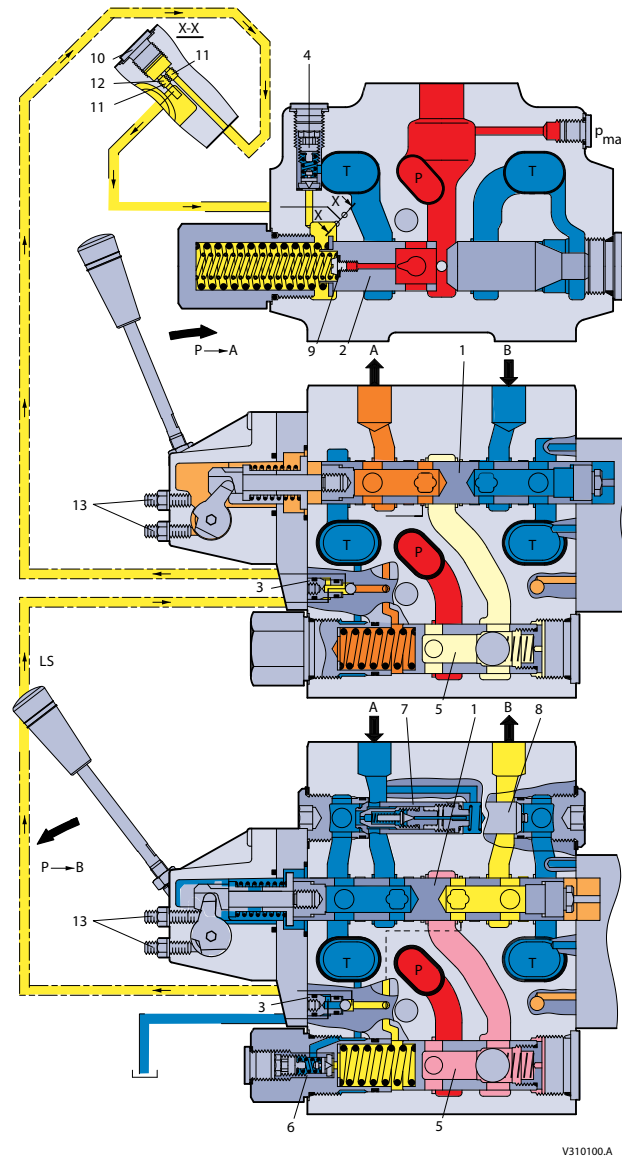
PVG 120 sectional view
