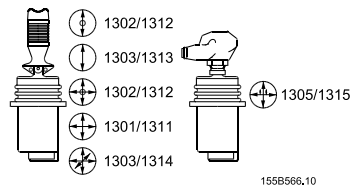
PVRE, electrical control unit, 162F...
