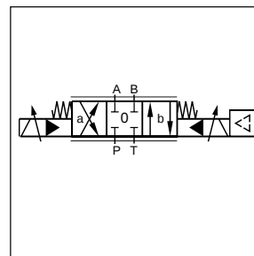
Standard D*1FB OBE
