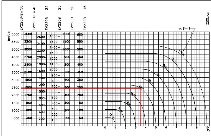
Figure 6: Capacity diagram
