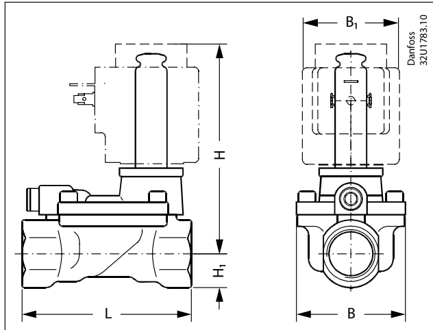
Figure 7: Dimension
