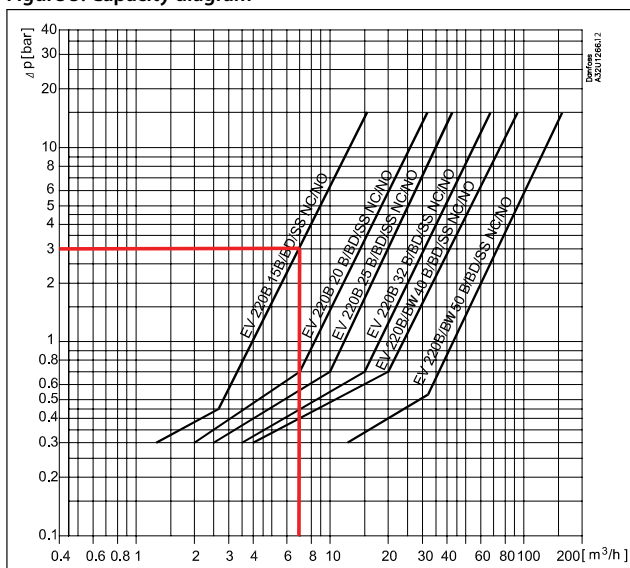
Figure 5: Capacity diagram
