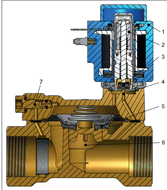
Figure 2: Function, NO
