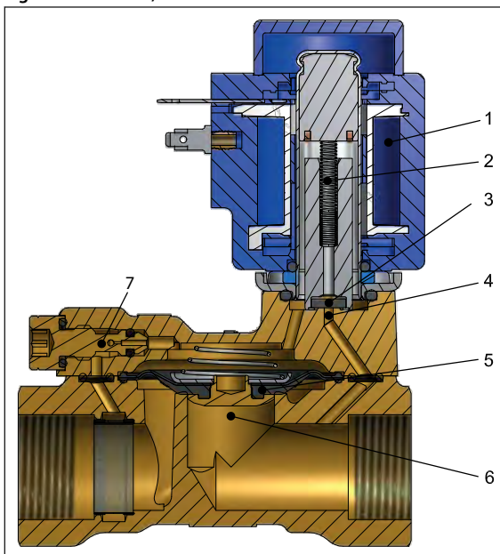
Figure 1: Function, NC
