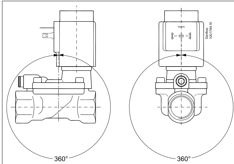
Figure 8: Mounting angle
