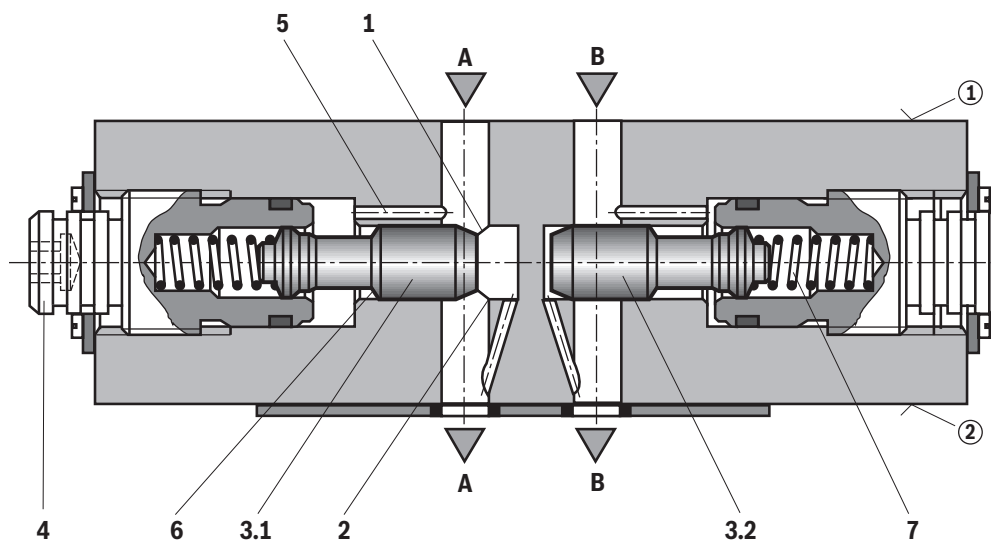
Supply throttling
