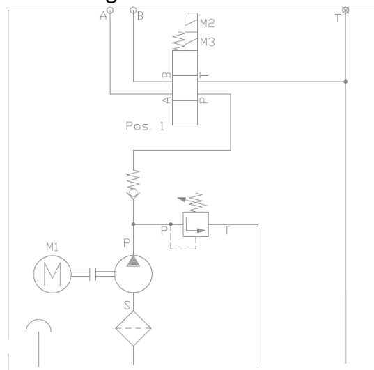
Circuit diagram:
