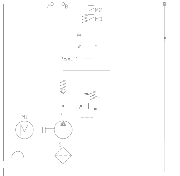
Circuit diagram:
