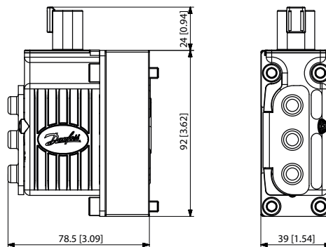
PVEA (-F) Series 6 dimensions
