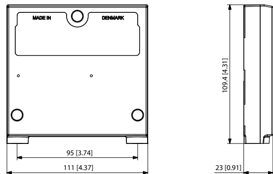
PVS/PVSI dimensions
