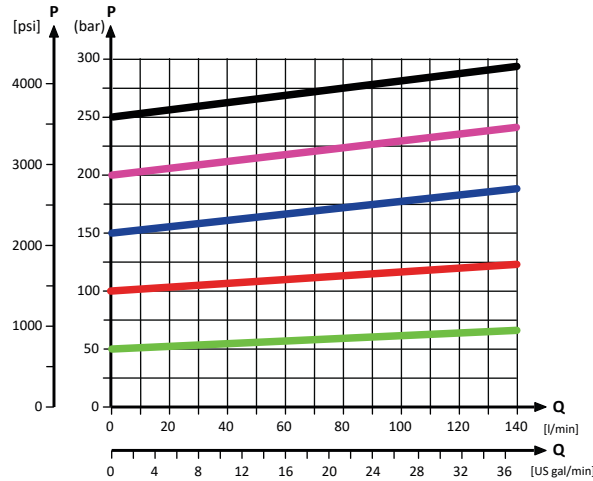
Neutral by-pass pressure drop characteristics
