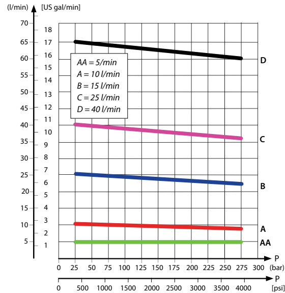
Load Independent Fluid Flow – Pressure Compensated PVB
