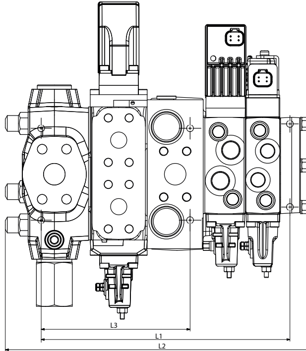
PVB 120/16 combination valve stack dimensions, mm [in]
