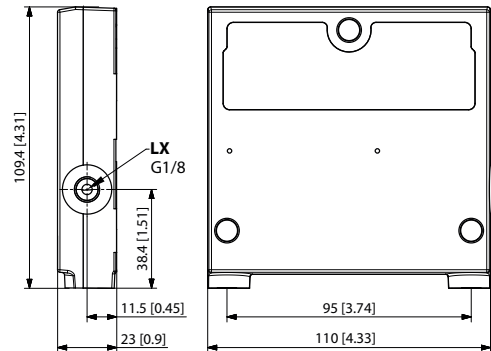
PVS/PVSI with LX-connection dimensions
