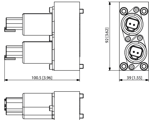
PVHC dimensions
