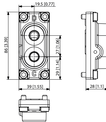
PVH 16 cover dimensions
