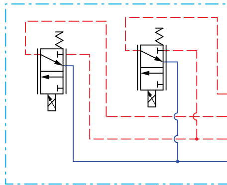
PVHC schematic
