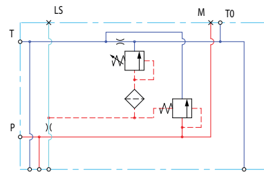
Open center PVP with T0
