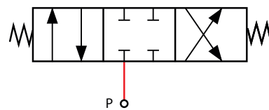
Uncompensated PVB schematic symbol
