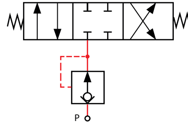
Compensated PVB schematic symbol
