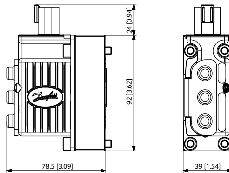
PVEO Series 6 dimensions
