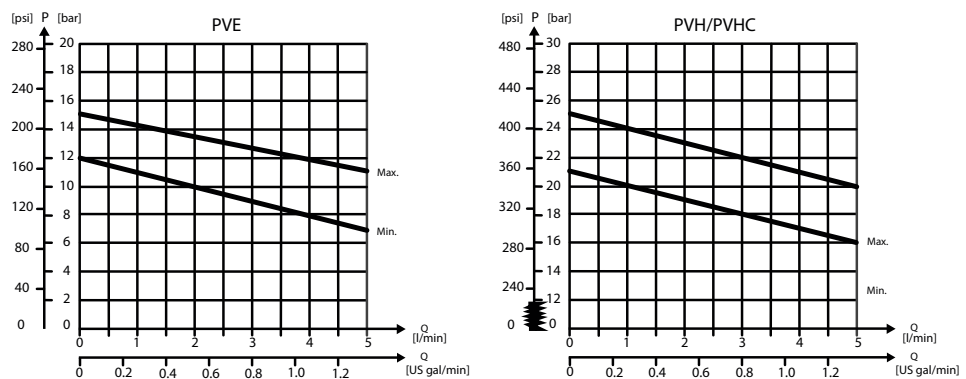
Pilot pressure reduction valve characteristics
