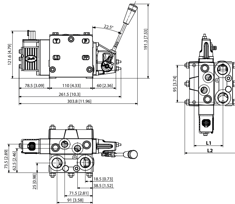
PVB 16 dimensions (12 sections)
