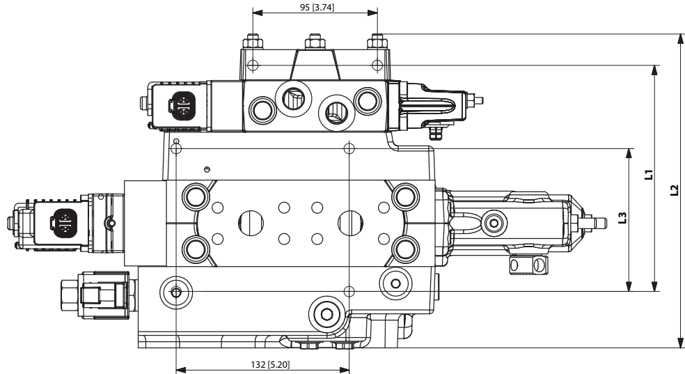
PVB 256/16 combination valve stack dimensions, mm [in]
