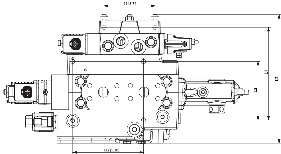
PVB 128/PVB 16 valve stack dimensions, mm [in]
