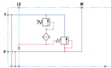
Open center PVP schematic
