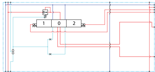
Compensated PVB schematic
