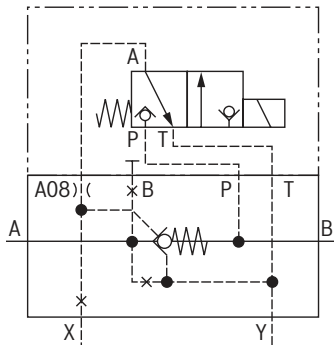
With directional seat valve type M-3SEW 6 C...
