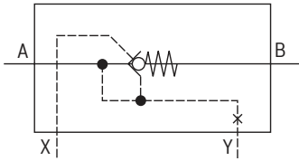
Version "SV" (internal pilot oil return)
