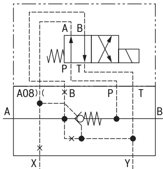
With directional spool valve type 4WE 6 D...
