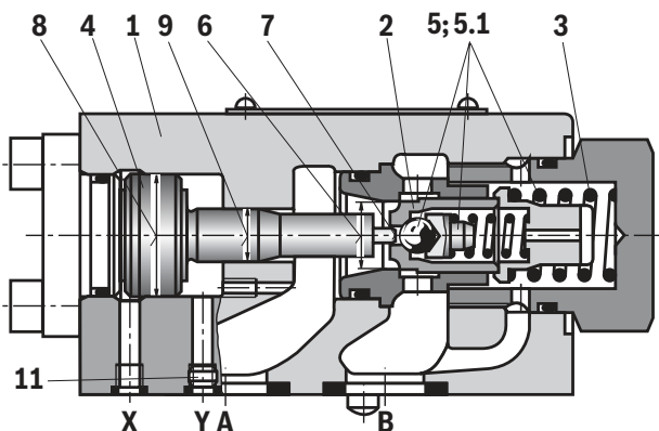
Type SV 10 PA.-4X... (without pilot oil return, with pre-opening)
