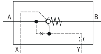
Version "SL" (external pilot oil return)
