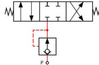
Compensated PVB schematic symbol
