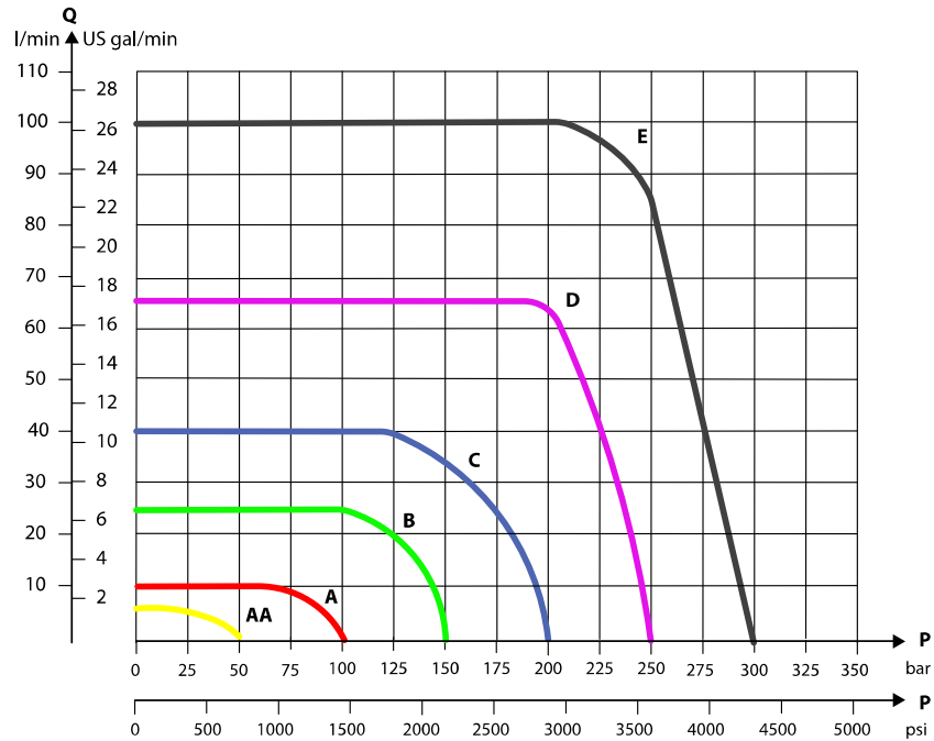
PVB pressure compensated for LS A/B characteristics
