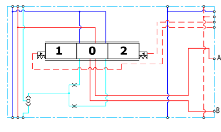
Uncompensated PVB with T0
