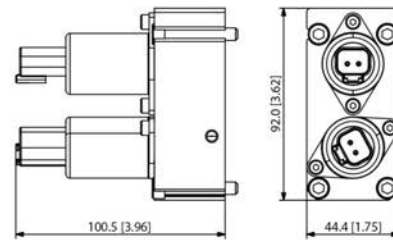
PVHC dimensions
