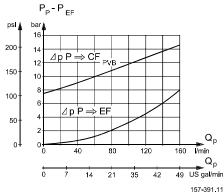
PVSP/PVSPM pressure drop characteristics
