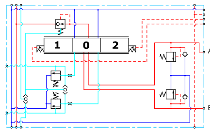
Compensated PVB with LS
