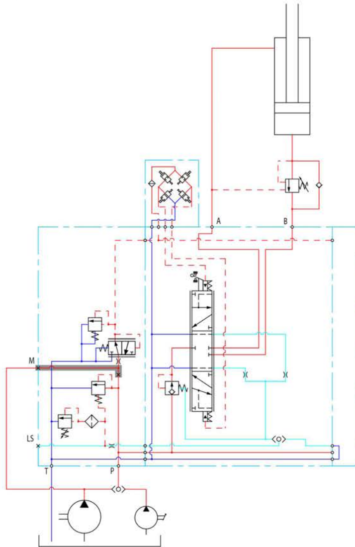
Hydraulic diagram for PVPC without check valve
