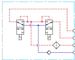
PVEO-HP Schematic
