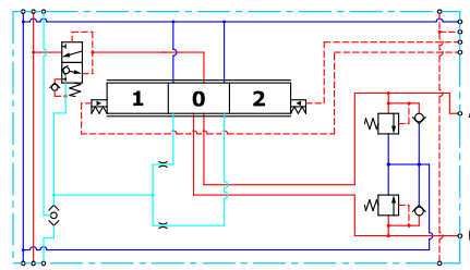
Compensated high flow PVB
