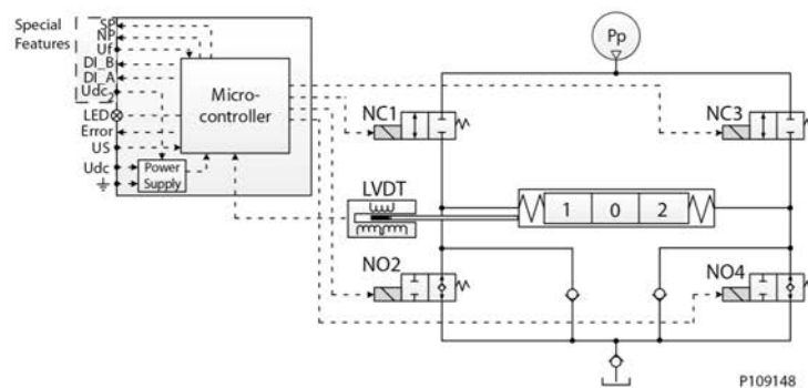
PVEH-NP functionality diagram
