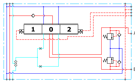
Uncompensated PVB with load drop check valve
