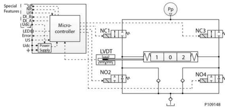
PVES-SP functionality diagram
