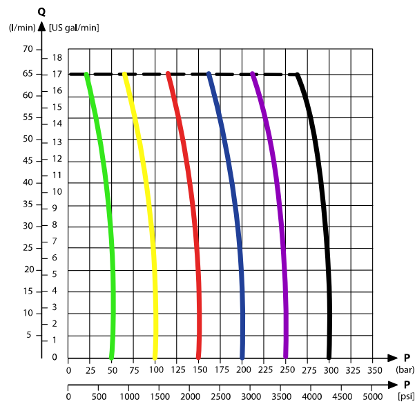
PVB pressure compensated for LS A/B characteristics
