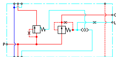
Open Center PVSPM giving priority to OSP+PVB
