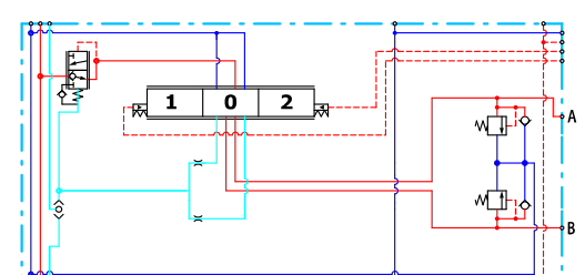
Compensated high flow PVB with T0
