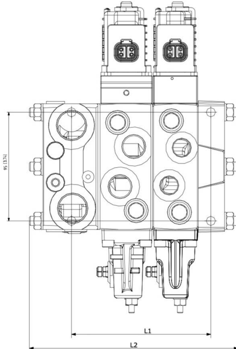
PVB 32/16 combination valve stack dimensions, mm [in]
