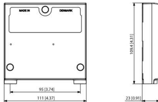
PVS/PVSI dimensions
