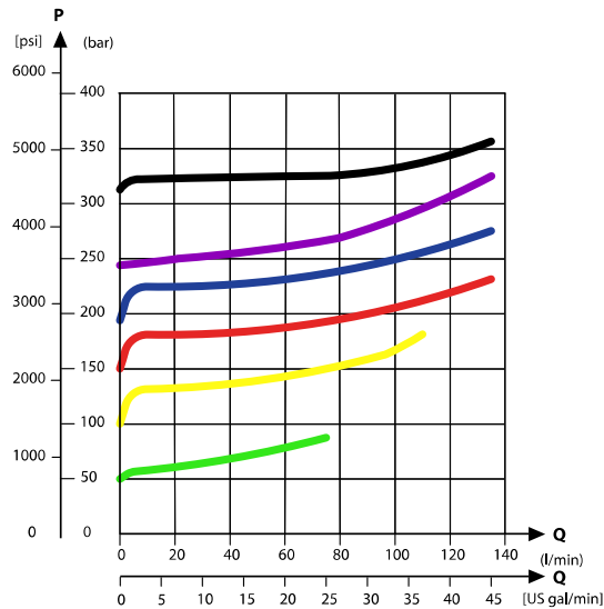
PVLP/PVLA suction valve characteristics
