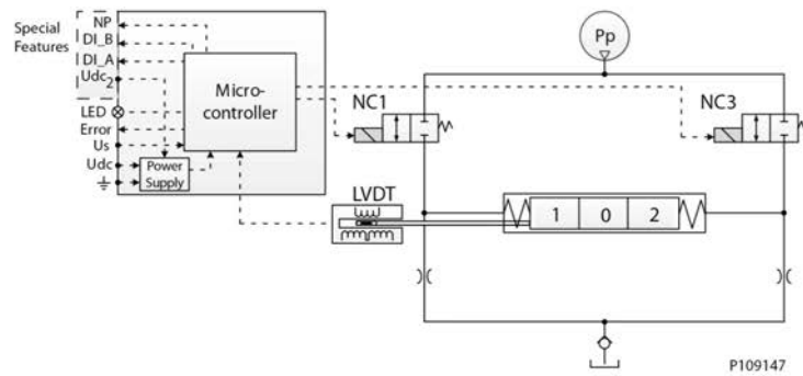
PVEH-NP functionality diagram
