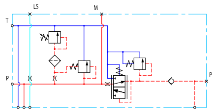
Closed center PVP with PPRV schematic
