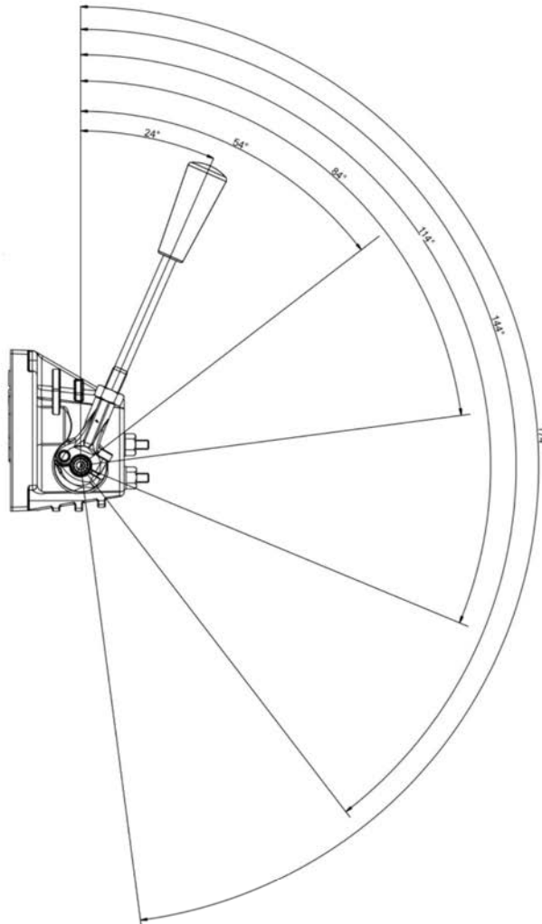
PVM handle positions
