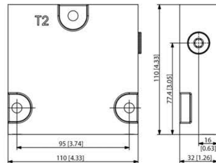
PVST with T-connection dimensions
