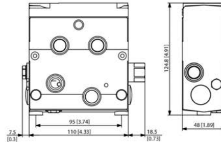
PVSP dimensions
