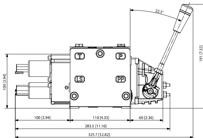
PVG 32 with PVHC
