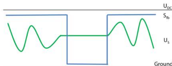
Solenoid disabling function (-NP) curves
