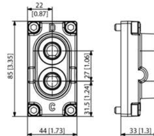
PVH 32 cover dimensions
