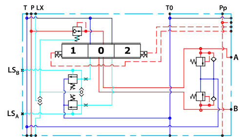
Compensated PVB with LS and T0
