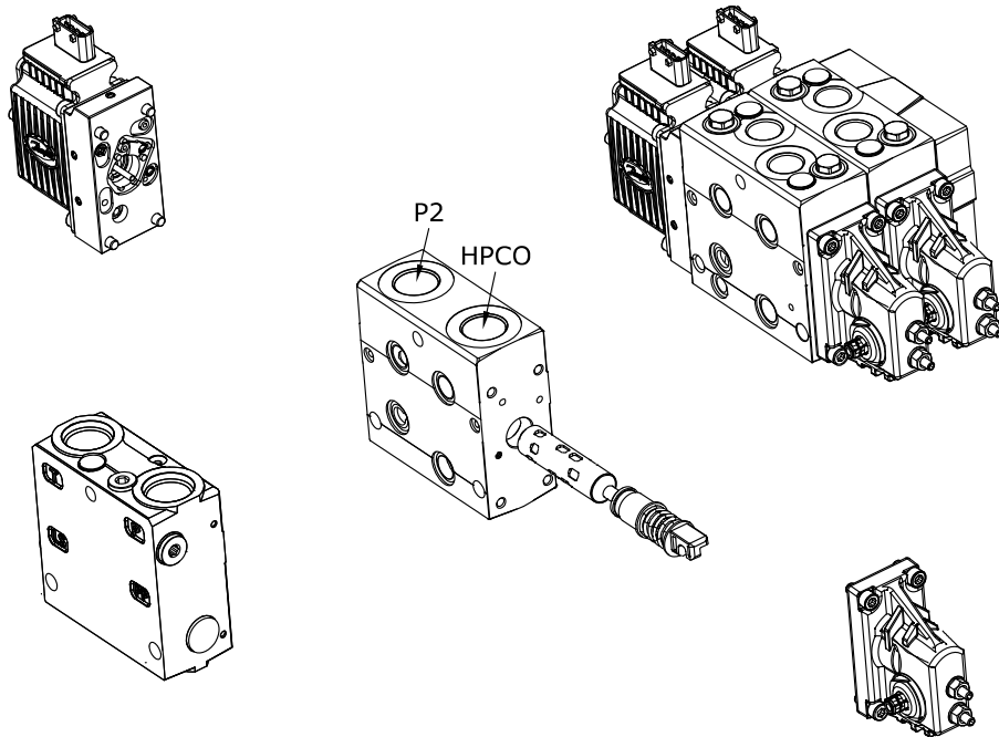
Optional mount of the PVSKM
