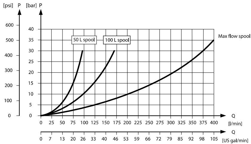
P-PVG flow
