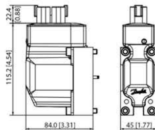
PVED-CC Series 5 dimensions
