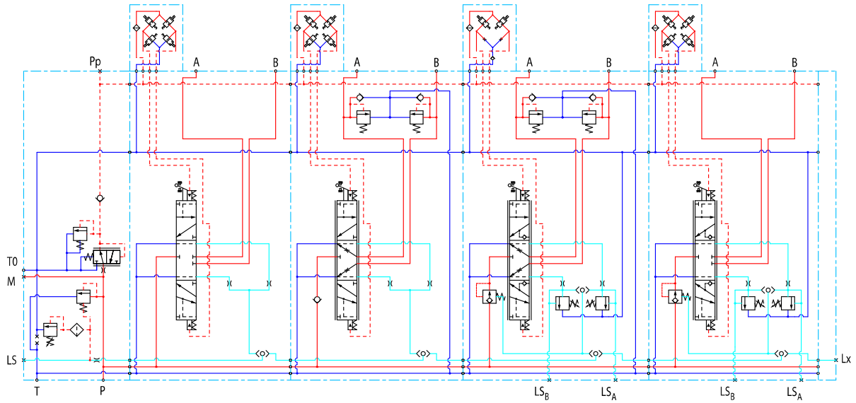
PVG with Open/Closed center PVP schematic
