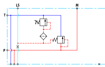
Open center PVP schematic
