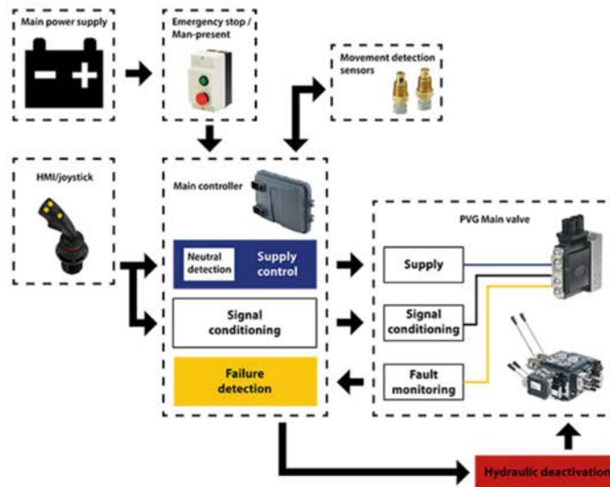
Electrical block diagram
