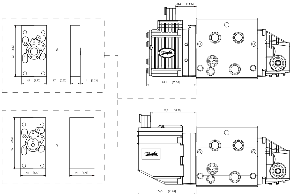
PVE Series 7 extension plates
