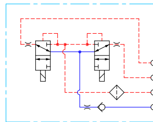
PVEO-R schematic
