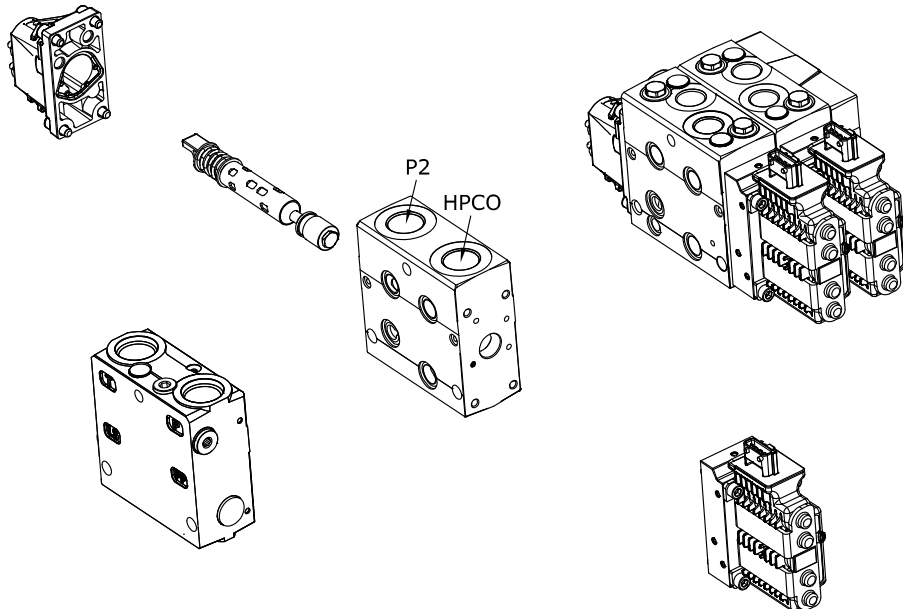
Optional mount of the PVSKM
