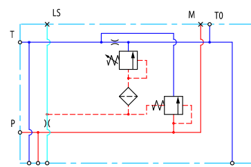
Open center PVP with T0
