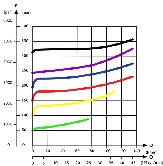
PVLP shock valve characteristics
