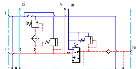
Closed center PVP with PPRV and T0
