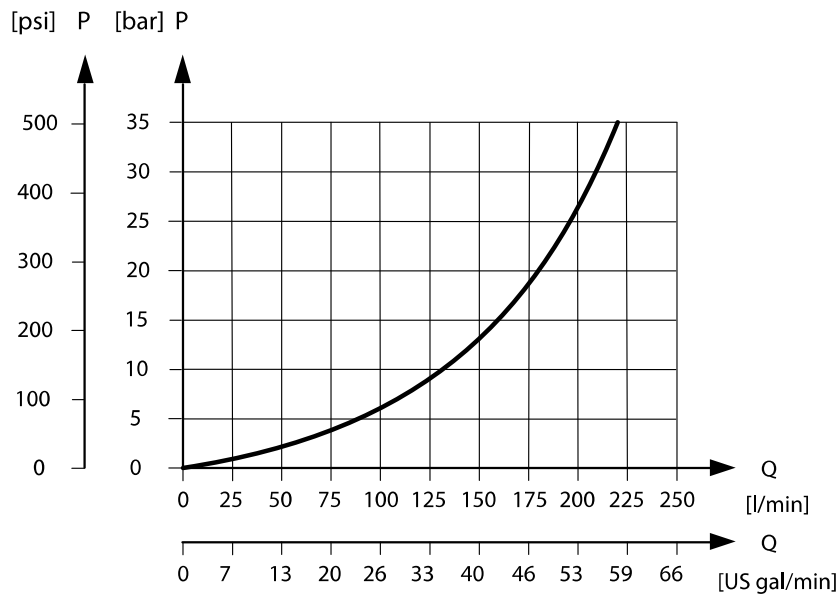
P-PVG flow
