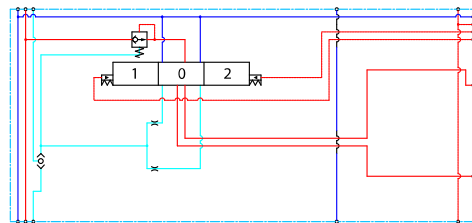
Compensated PVB schematic
