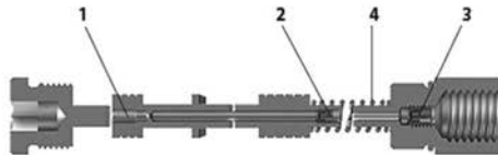
Compensator spool sectional view
