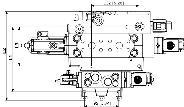
PVB 128/32 combination valve stack dimensions, mm [in]
