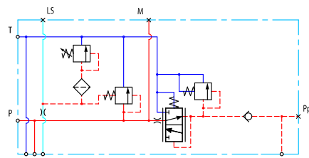
Open center PVP with PPRV schematic
