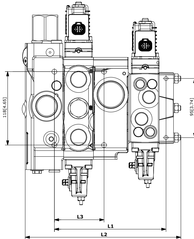
PVB 100/32 combination valve stack dimensions, mm [in]
