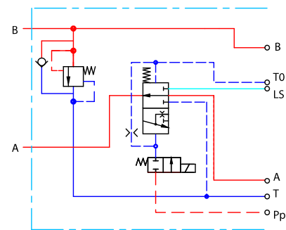
Multi-valve schematic
