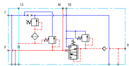
Open center PVP with PPRV and T0
