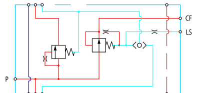
Closed Center PVSPM giving priority to OSP+PVB
