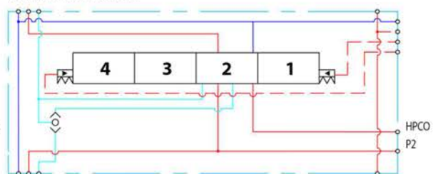
Schematic without T0
