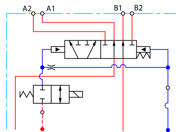
PVBD schematic
