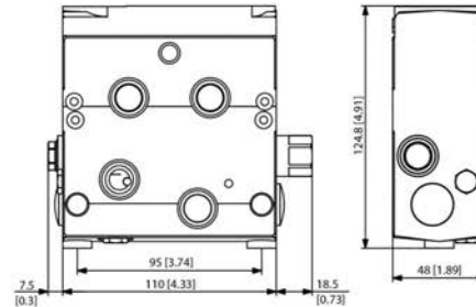
PVSPM dimensions
