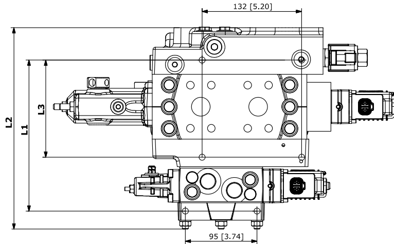
PVB 256/32 combination valve stack dimensions, mm [in]
