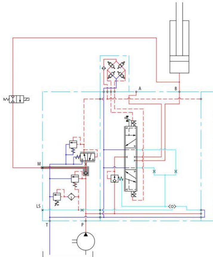
Hydraulic diagram for PVPC with check valve
