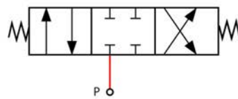
Uncompensated PVB schematic symbol
