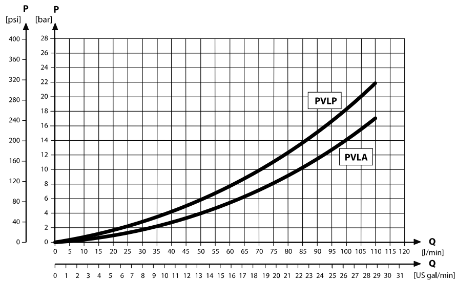
PVLP/PVLA suction valve characteristics
