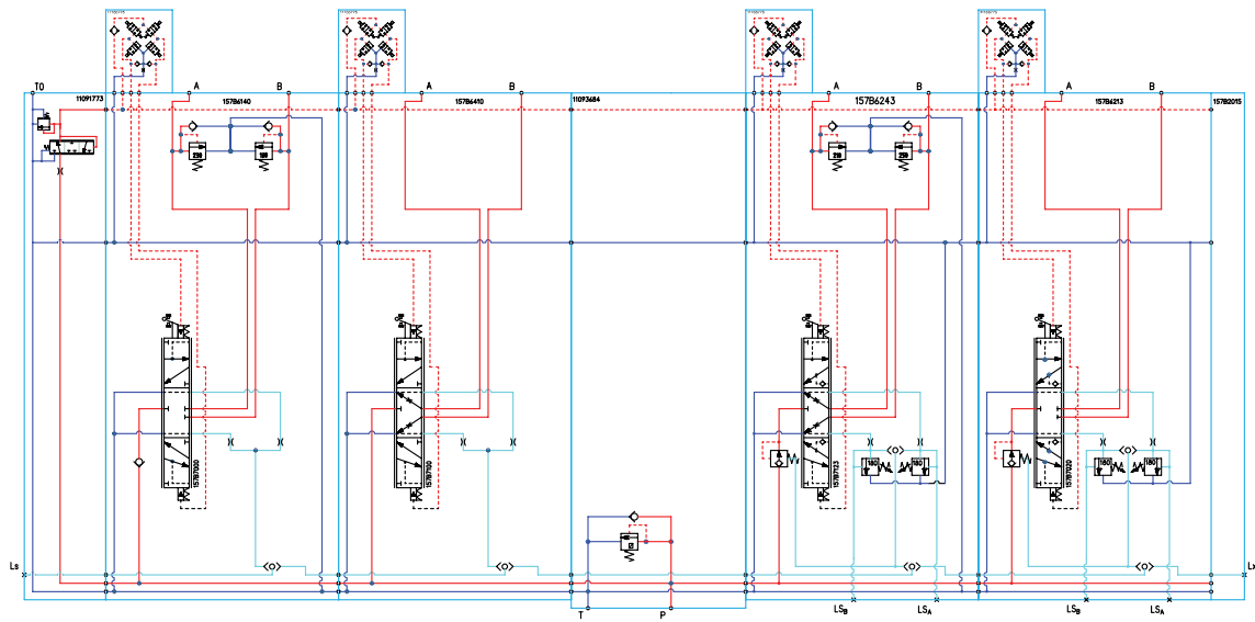
PVG with Open/Closed center PVP schematic
