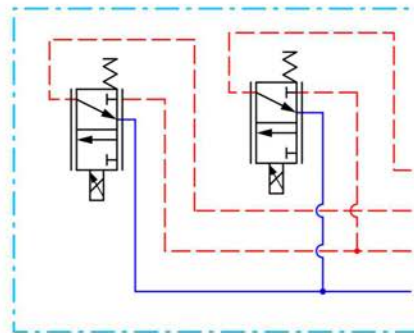
PVHC schematic
