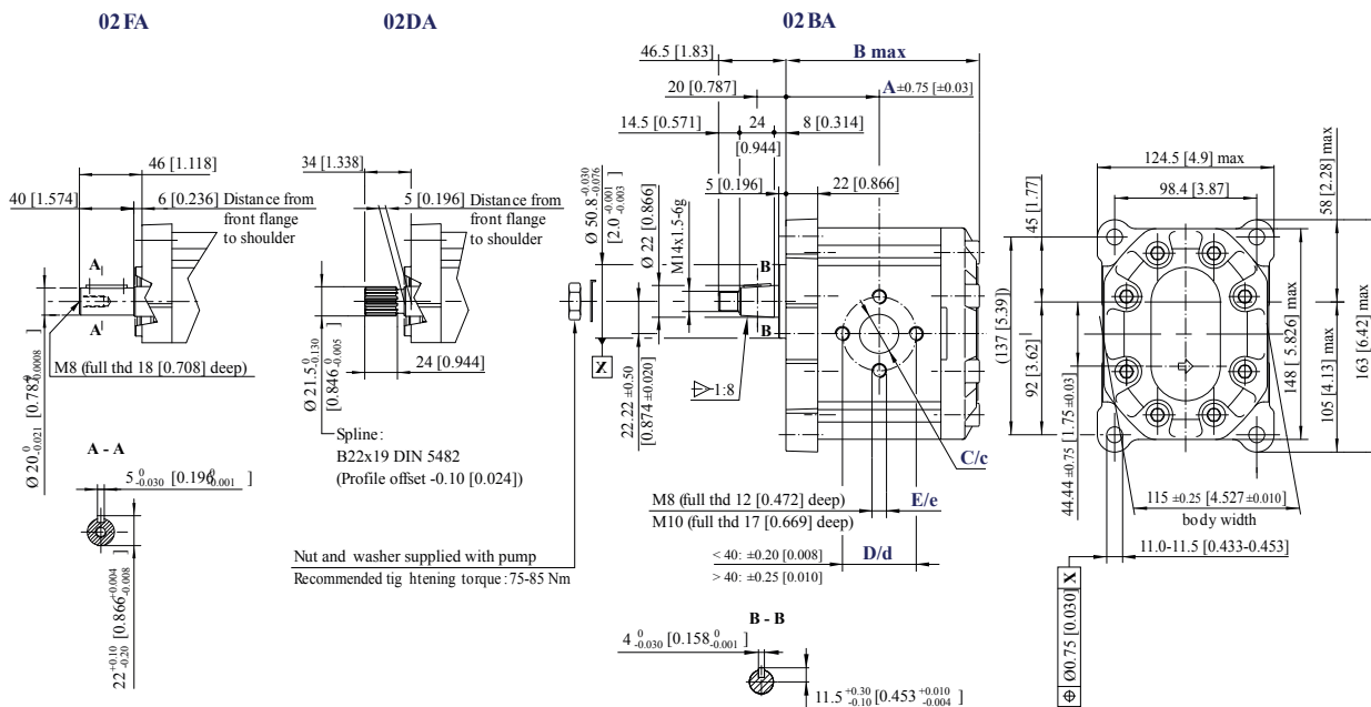
SNP3NN - 02FA, 02DA AND 02BA dimensions
