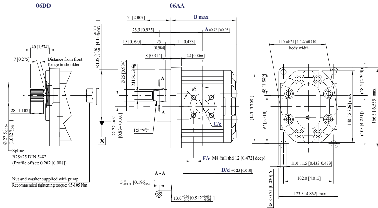
SNP3NN – 06DD and 06AA dimensions
