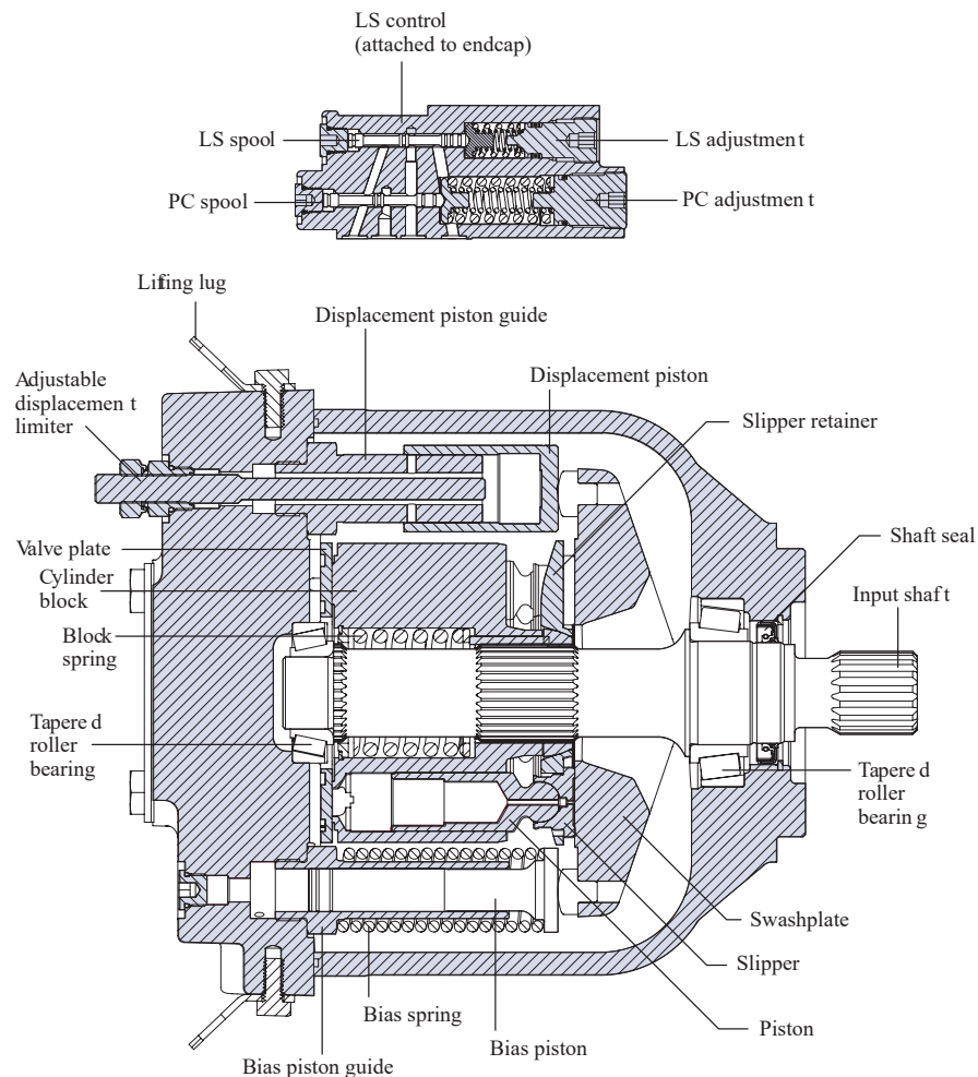
Frame E cross section
