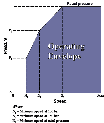
Speed versus pressure
