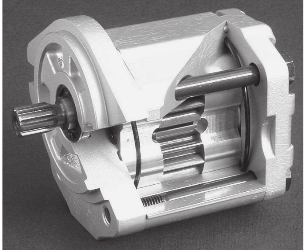
SNP2NN 06SA cut-away
