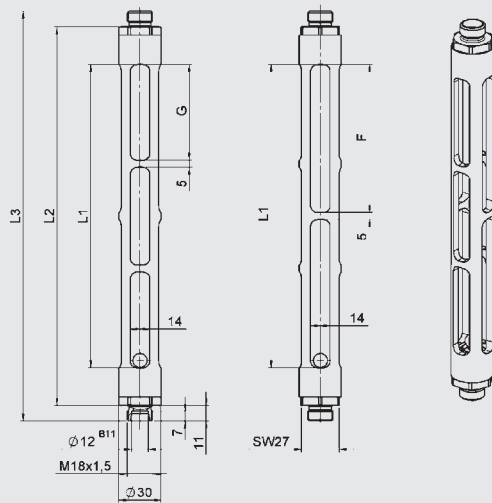
FSAR without mounting nut
