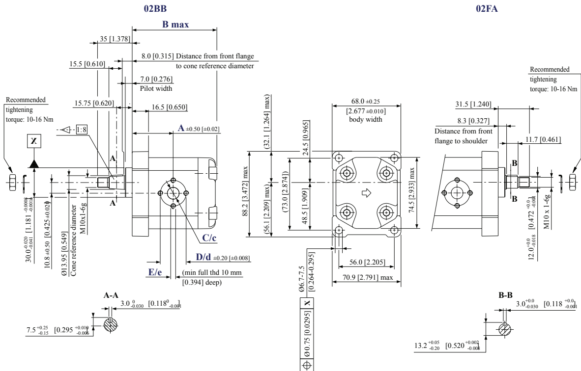
SKP1NN – 02BB and 02FA dimensions
