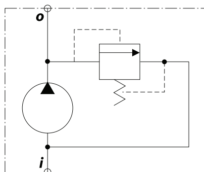
Valve schematic
