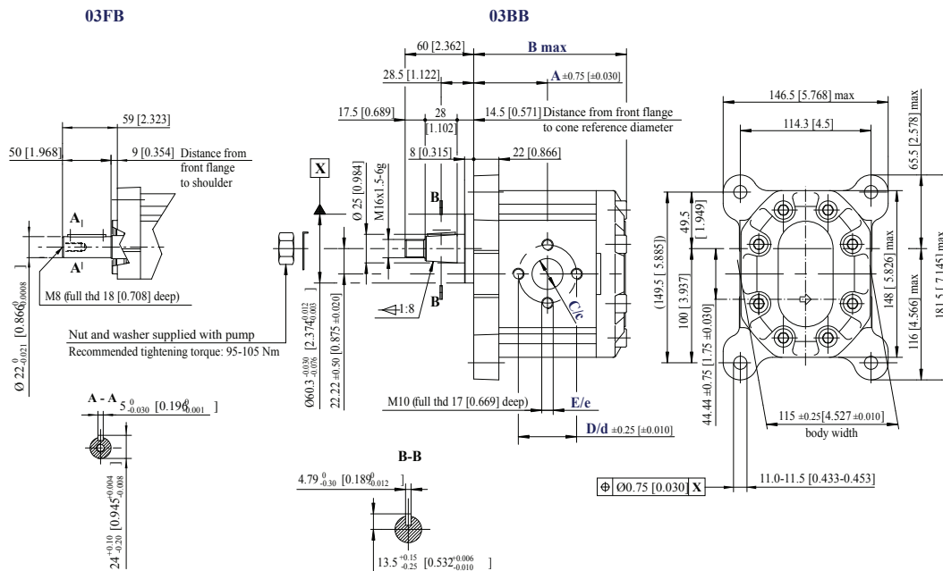
SNP3NN – 03FB and 03BB dimensions
