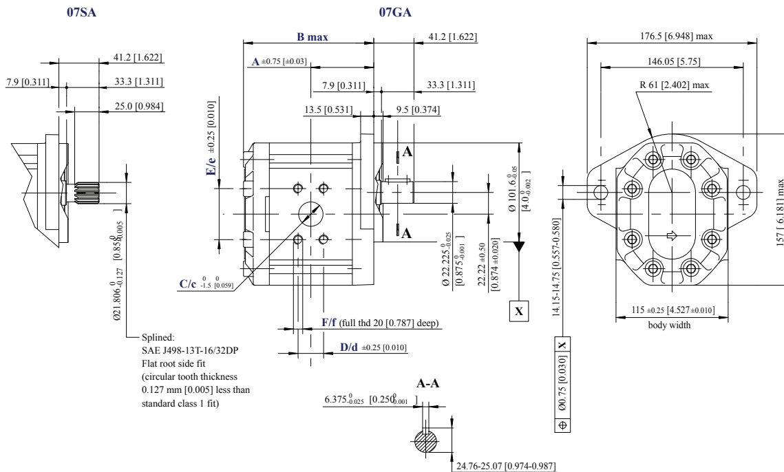
SNP3NN – 07SA and 07GA dimensions
